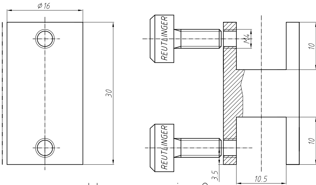
assembly accessories 2x scale 1:1
